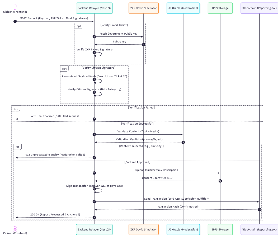
Figure 3.10: Backend relay workflow architecture.
